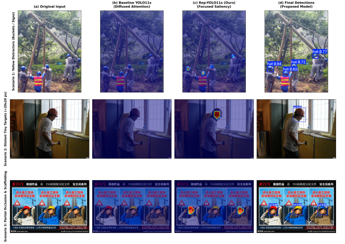
Fig. 4. Visual Saliency Map Comparison using Grad-CAM across complex construction scenarios: Row 1 (Yellow Distractors), Row 2 (Distant Tiny Targets < 20 \times 20 px), and Row 3 (Partial Occlusion). (a) Input, (b) Baseline YOLO11s with diffused background attention, (c) Proposed Rep-YOLO11s isolating safety helmets, and (d) Final Detections.
